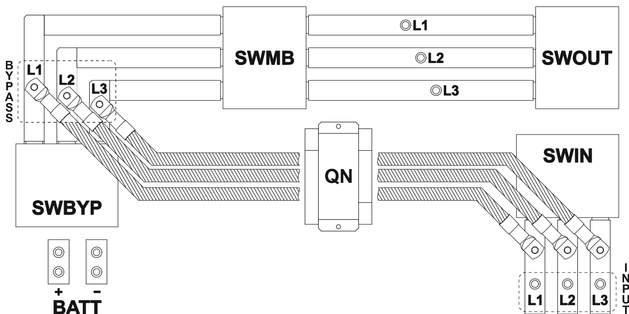
125KVA - DUAL INPUT
