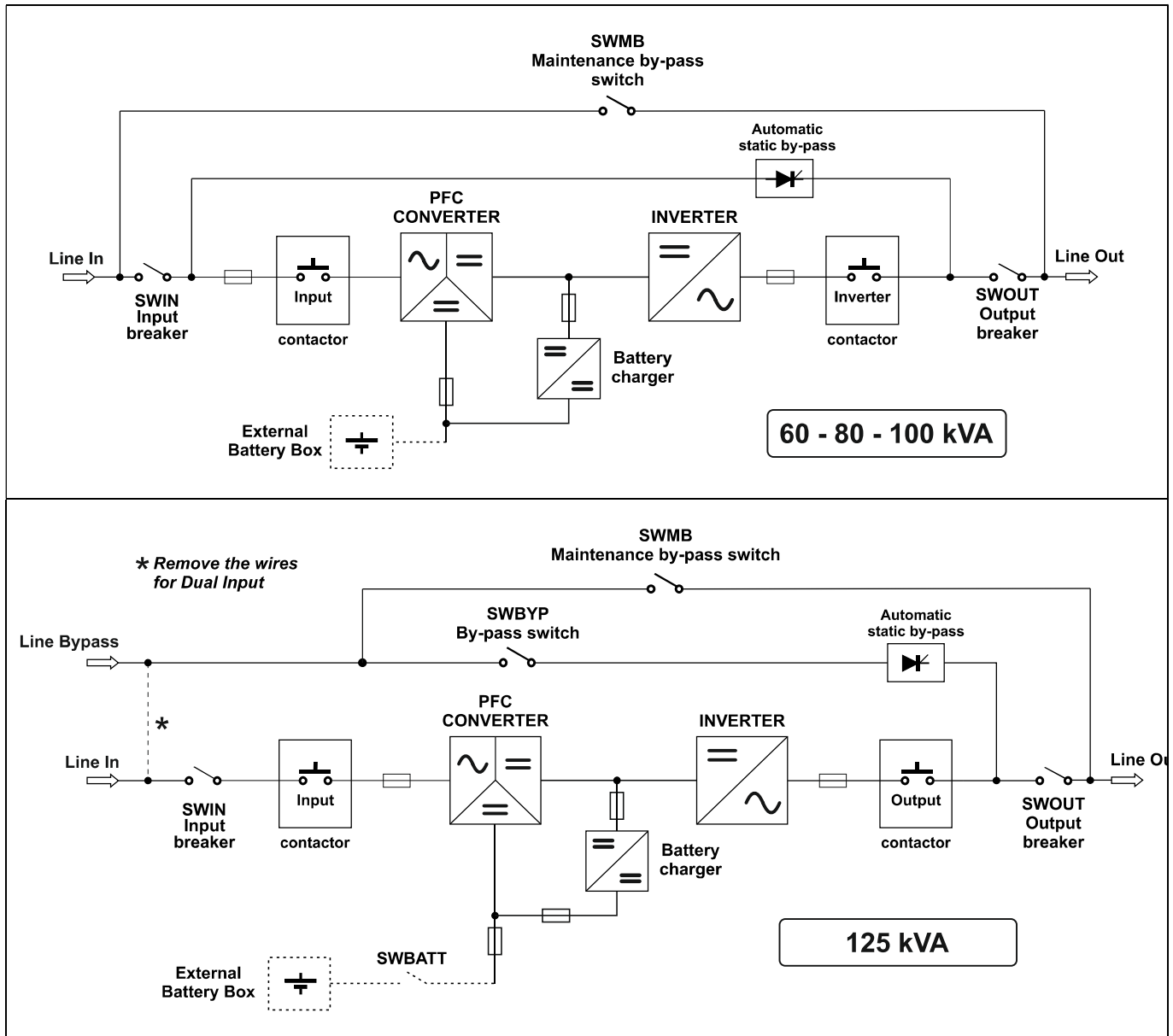
UPS block diagram
